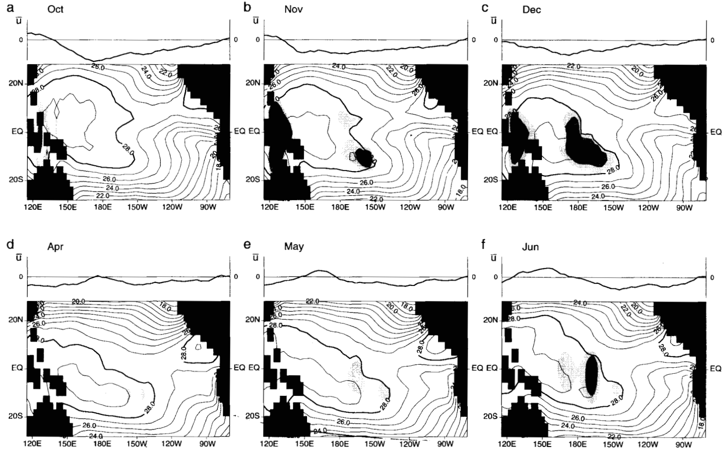
Figure 5. Contour maps of the observed monthly mean SST in the tropical Pacific Ocean during October, November and December (OND) and April, May and June (AMJ). Superimposed on each map are shaded contours of \delta E_{mc} for the fastest growing 'advection' singular vector (ASV) during the OND and AMJ quarters. Also shown are profiles of the monthly mean zonal ocean current \bar{u} at the equator. The contour interval for SST is 1°C, and a change in grey scale for \delta E_{mc} corresponds to an interval of 1.5 \times 10^{-2} non-dimensional units. The 28°C isotherm is highlighted.
