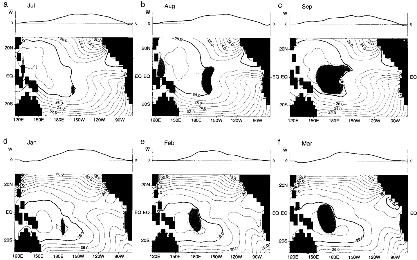
Figure 4. Contour maps of the observed monthly mean SST in the tropical Pacific Ocean during July, August and September (JAS), and January, February and March (JFM). Superimposed on each map are shaded contours of \delta E_{mc} for the fastest-growing 'upwelling' singular vector (USV) during the JAS and JFM quarters. Also shown are profiles of the monthly mean vertical velocity \bar{w} at the equator. The contour interval for SST is 1°C, and a change in grey scale for \delta E_{mc} corresponds to an interval of 1.5 \times 10^{-2} non-dimensional units. The 28°C isotherm is highlighted.
