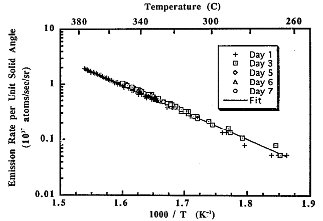
FIG. 2. Sodium emission rate per unit solid angle as a function of temperature. The different sets of data points correspond to different series of measurements and show the stability of the source. Note the exponential dependence on inverse temperature.
