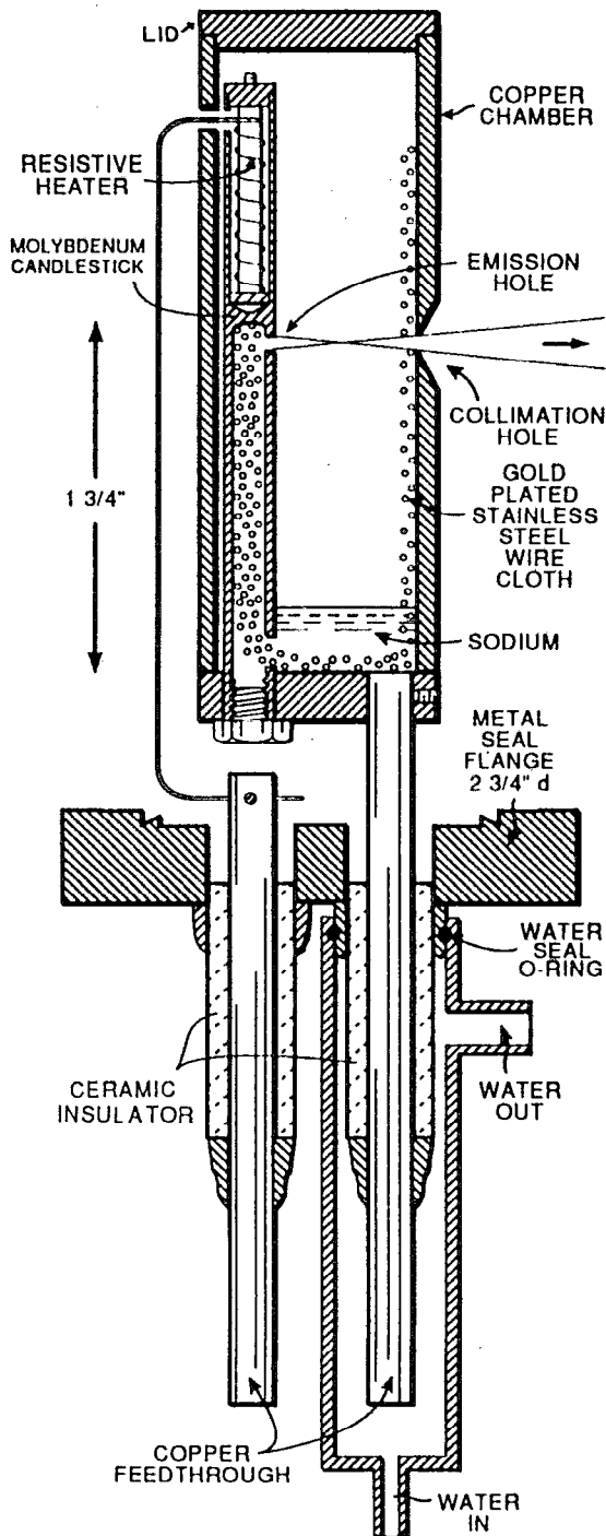
FIG. 1. Cross-sectional view of the candlestick atomic beam source. The assembly is mounted on one flange and fits inside a 2 3/4 in. UHV cross.
