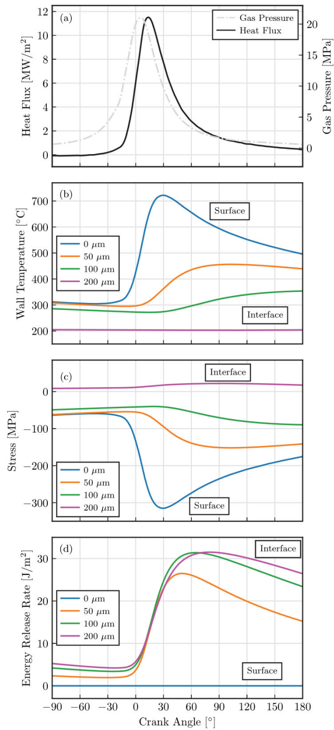
Fig. 4. Crank resolved evolution combustion chamber cylinder pressure (gray) and heat flux (black) (a), wall temperature distribution (b), x -direction stress distribution (c) and elastic energy release rate distribution (d) are shown during an engine cycle for the Rated Power condition. The surface (blue), 50 \mu\text{m} (orange), 100 \mu\text{m} (green) and interface 200 \mu\text{m} (pink) is depicted on (b), (c) and (d). Stress-free temperature and coating thickness was held constant at 230 °C and 200 \mu\text{m} , respectively. The Rated Power engine condition specifications and the thermomechanical properties of YSZ/Steel can be found in Table 1 and 2, respectively.
