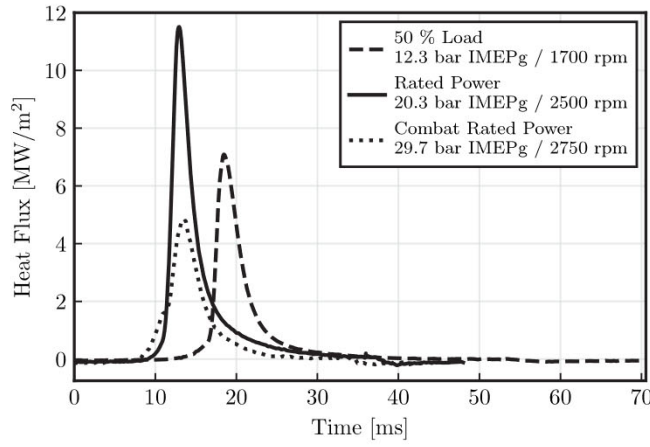
Fig. 2. Experimental area-weighted heat fluxes obtained via telemetry measurements on an uncoated-piston. Details of the engine operating conditions can be found in Table 1.
