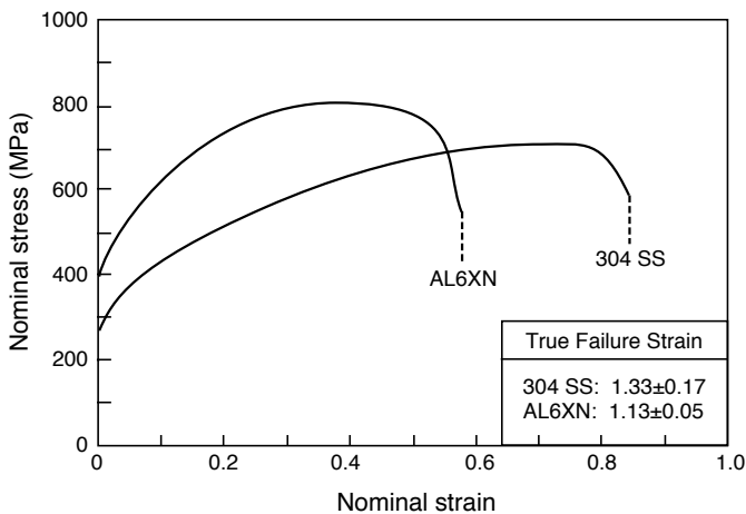
Figure 10. Quasistatic tensile stress-strain curves of both materials. Failure strains were calculated from area measurements at the fracture plane.
