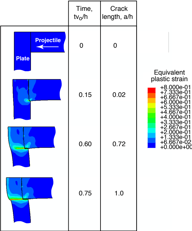
Figure 12. Evolution of plastic strain and crack growth for a 3 mm thick AL6XN plate impacted by a projectile with initial velocity v_o = 300 \text{ m/s} .
