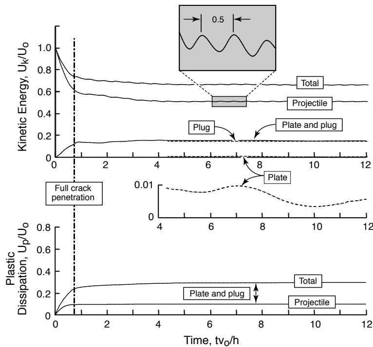
Figure 13. Evolution of kinetic energy and plastic dissipation during a shear out test (AL6XN, h = 3 mm, v_o = 300 m/s, \varepsilon_f = 0.8 ). Insets in the top graph illustrate the oscillatory nature of projectile and plate kinetic energies as well as the pertinent time scales. U_o is the initial projectile kinetic energy.
